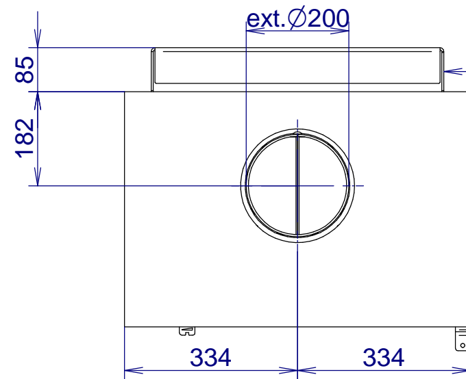
VENUS 630DC V23 in the box + console for wall
